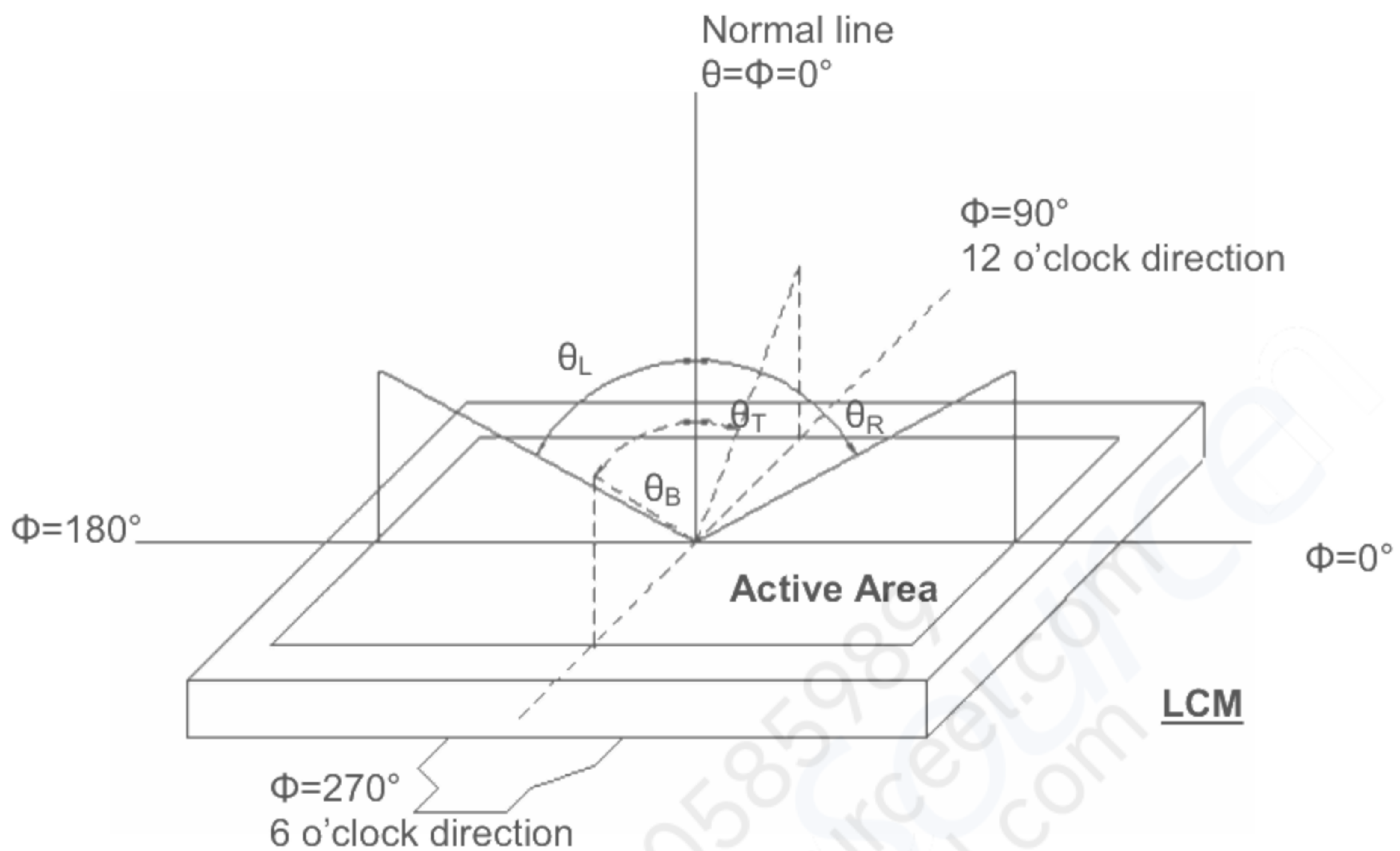
Fig. 4-1 Definition of viewing angle
