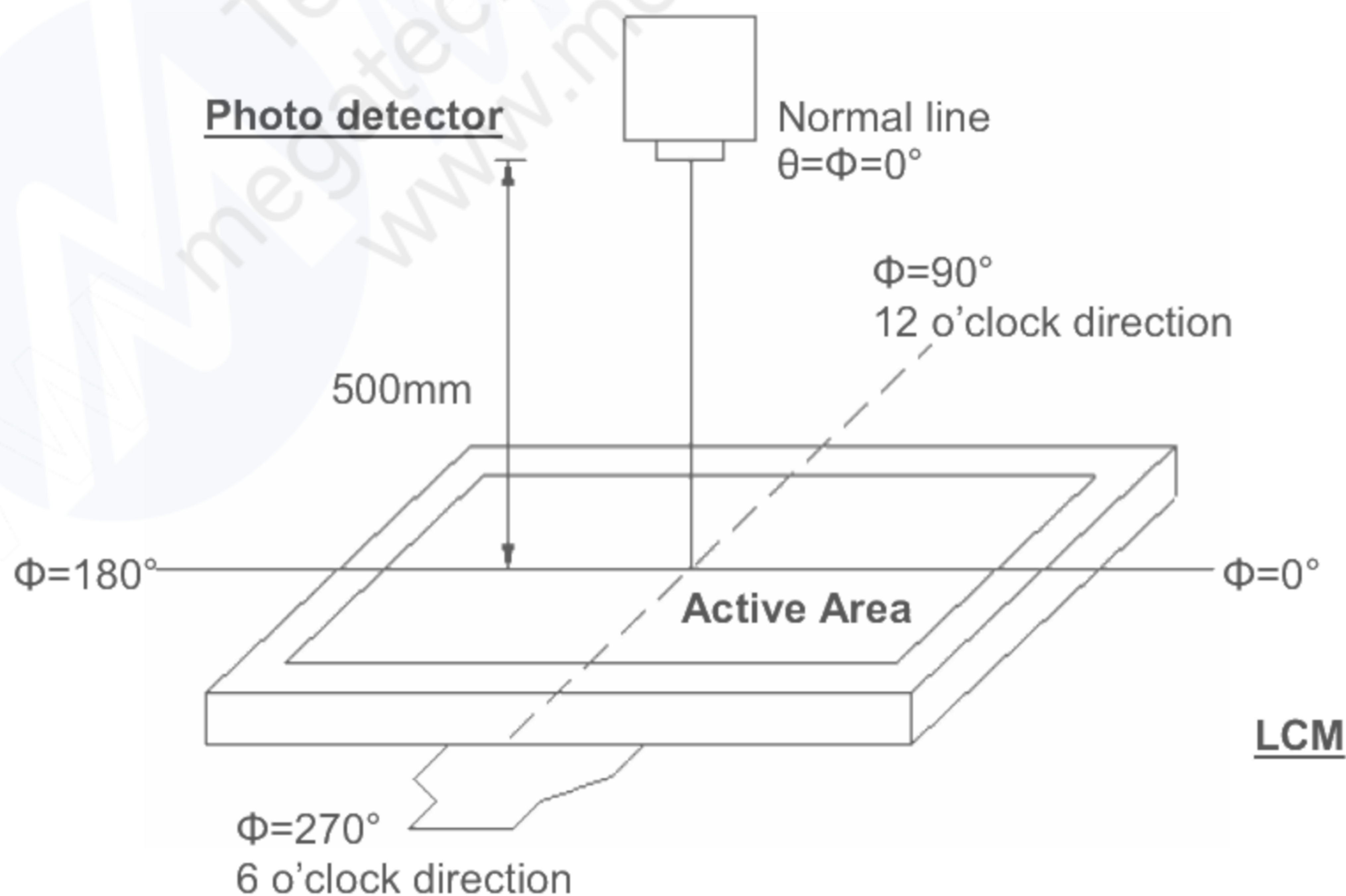
Fig. 4-2 Optical measurement system setup
