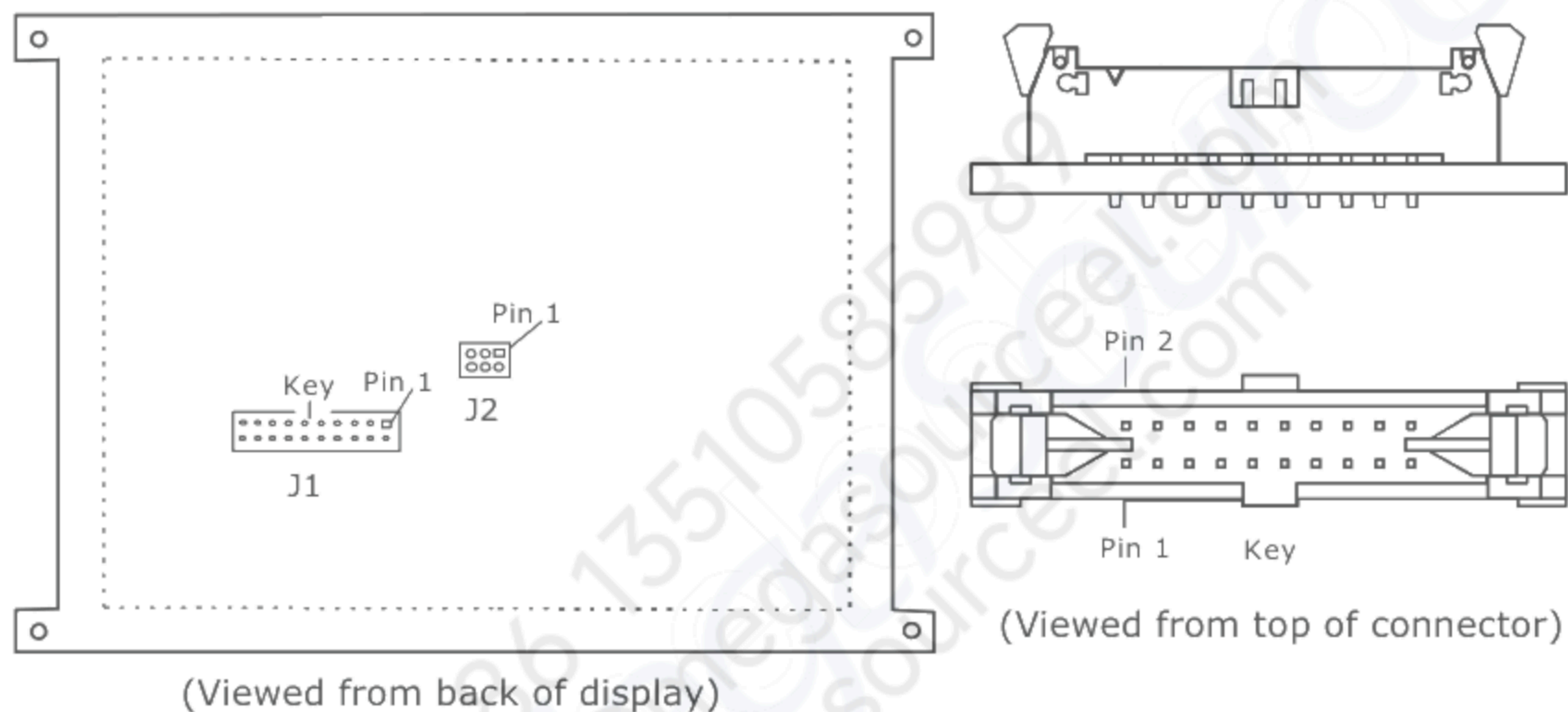
Figure 1. Data/power connector
