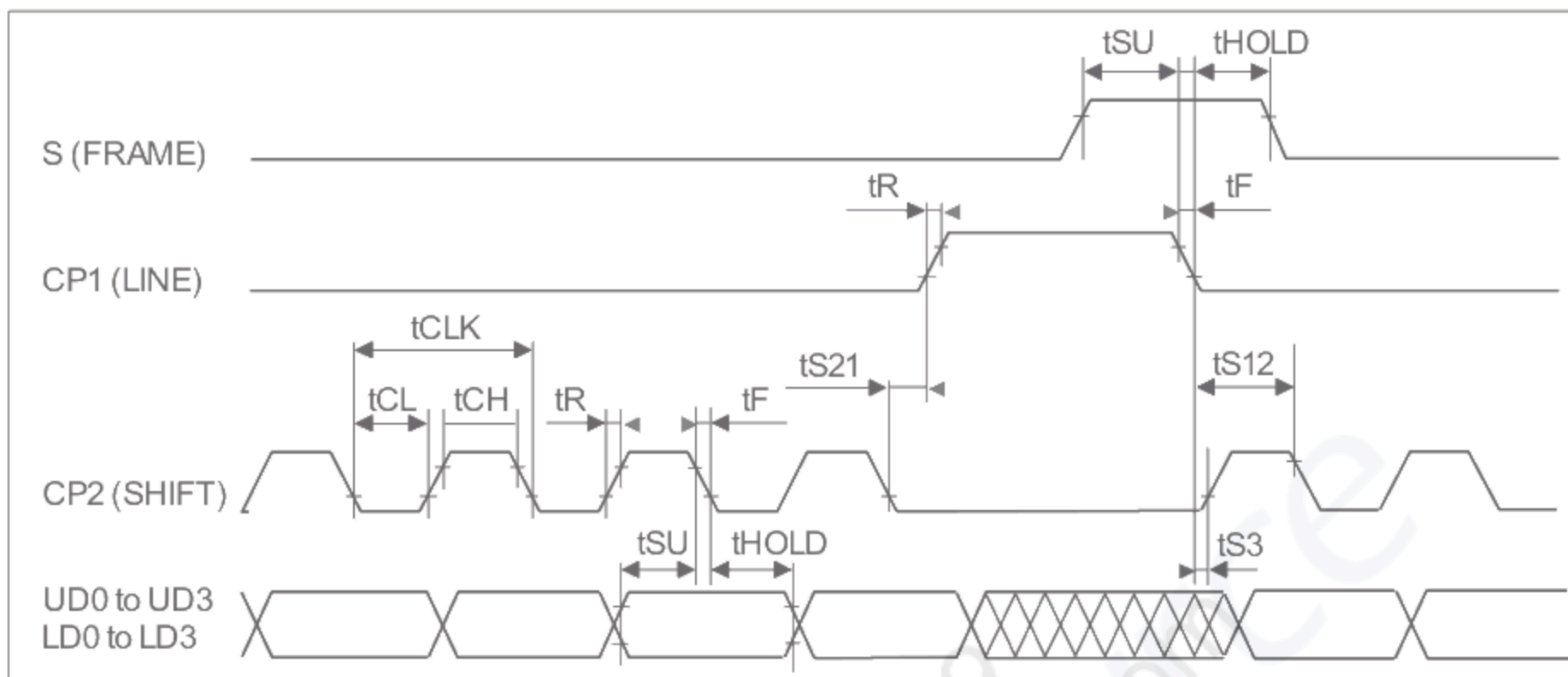
Figure 3. Setup and hold timing diagram
