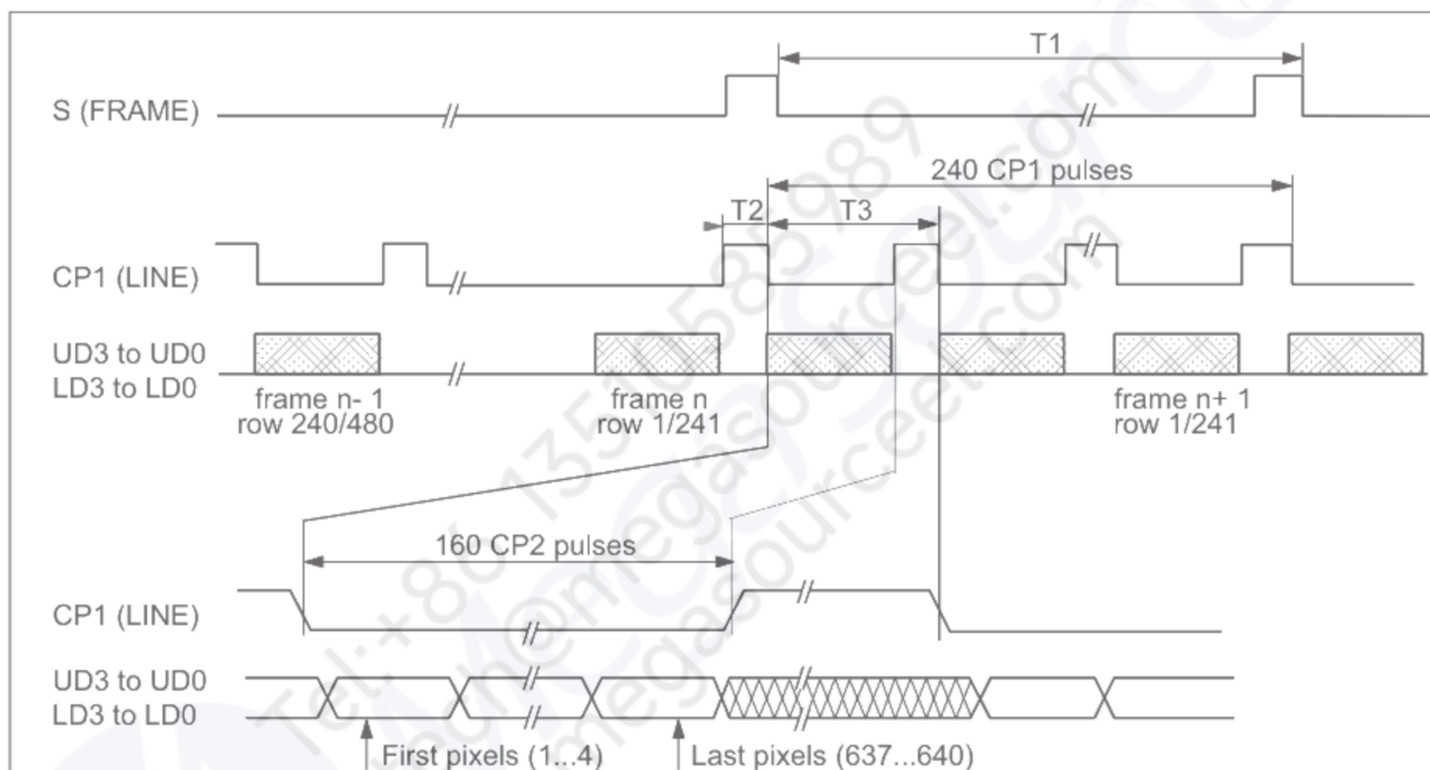
Figure 2. Video input timing diagram
