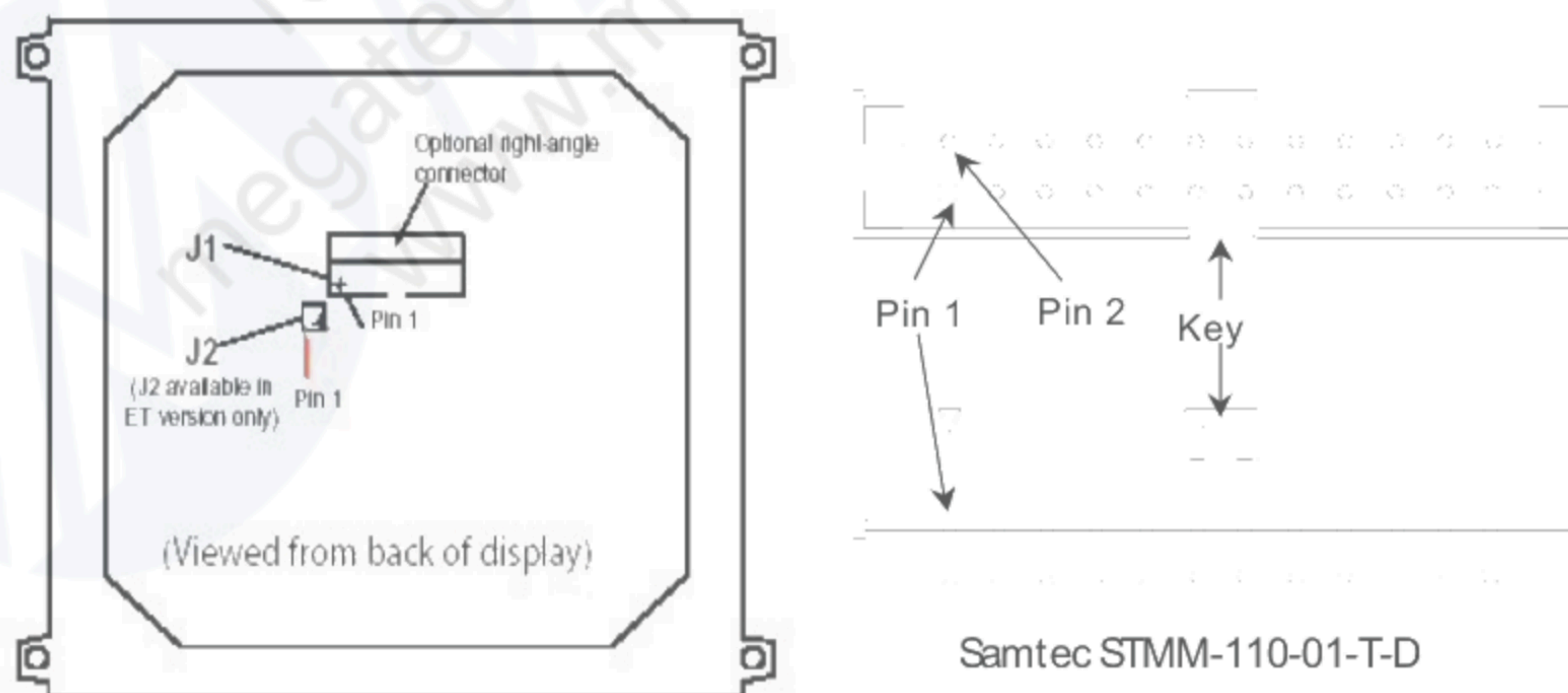
Figure 1. Data/power connector
