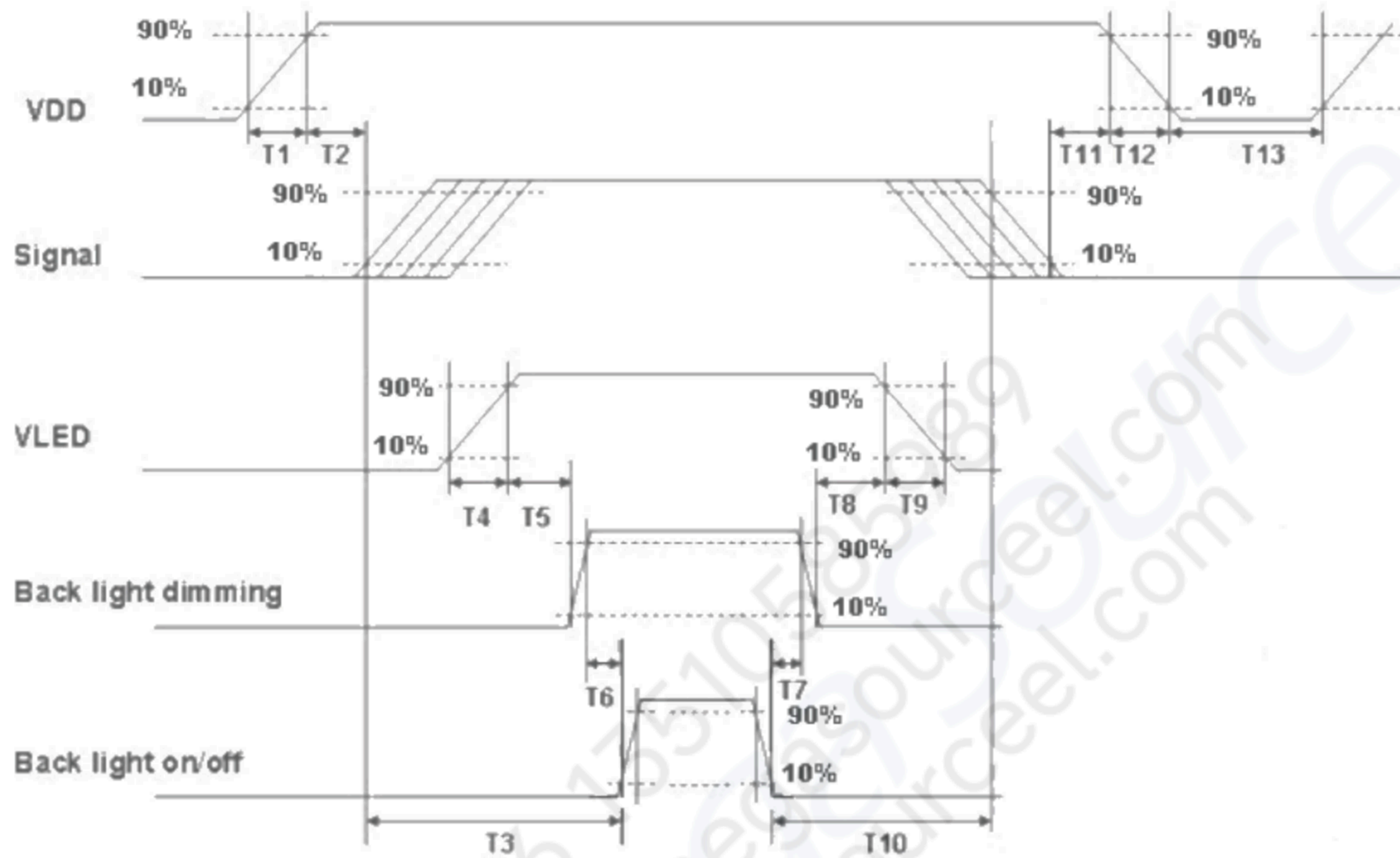
Power Sequence Timing
