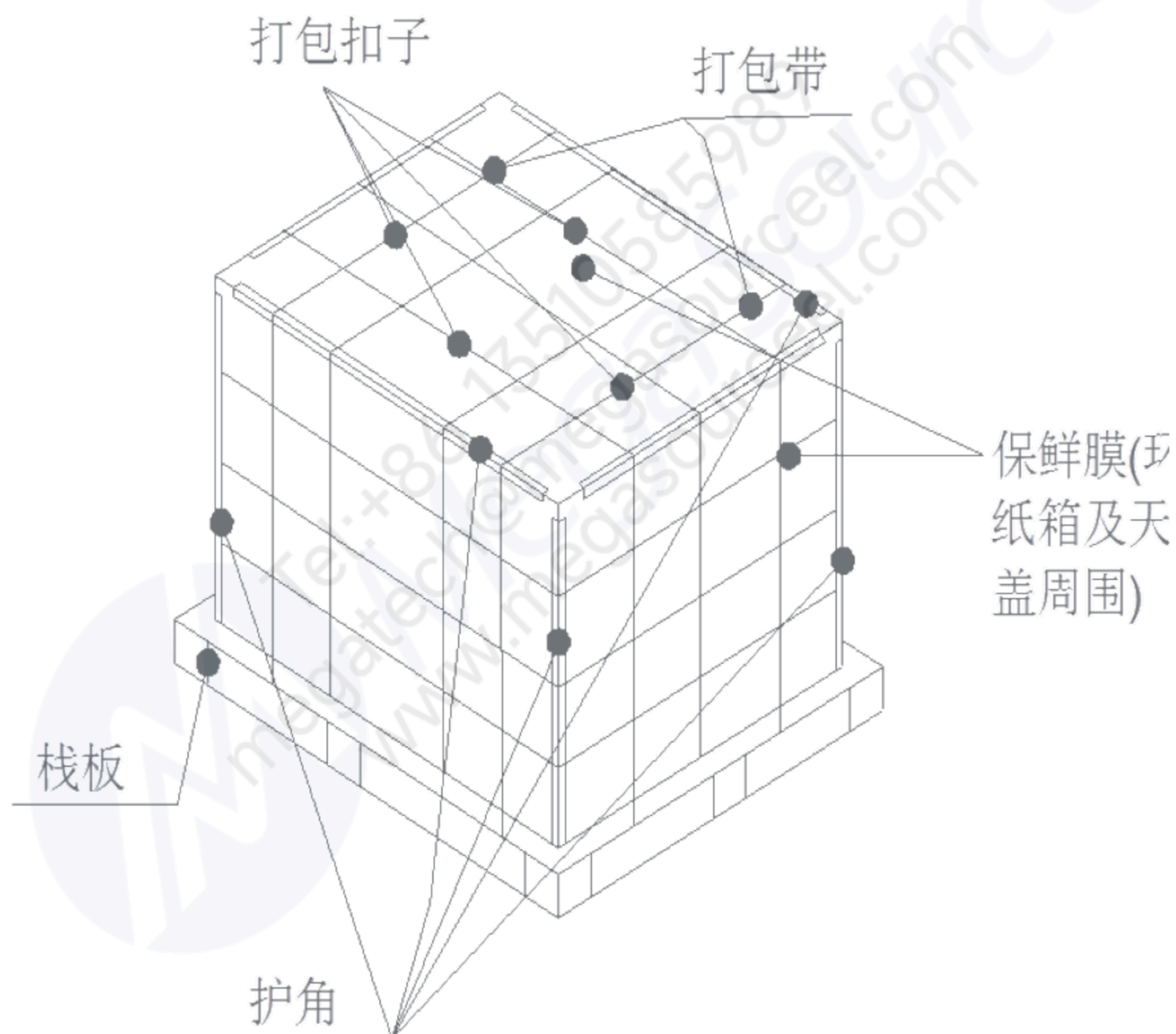
Figure 9. Packing Method
