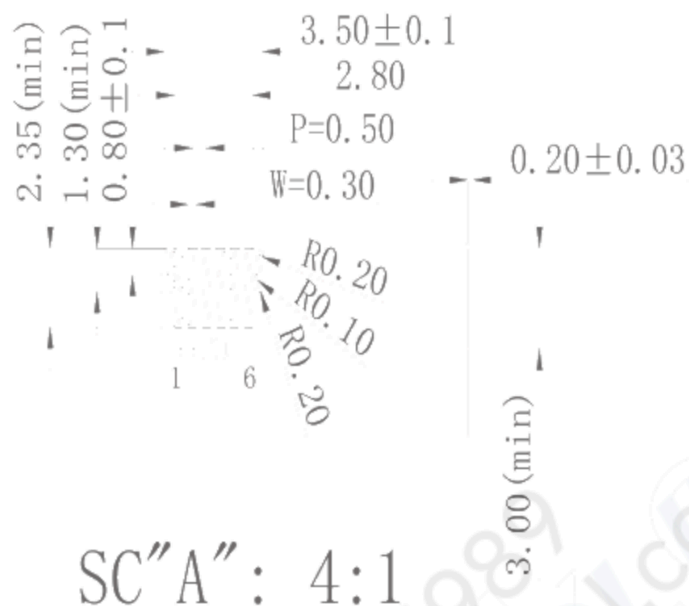
Figure 8. LCM Outline Dimension (unit: mm)
