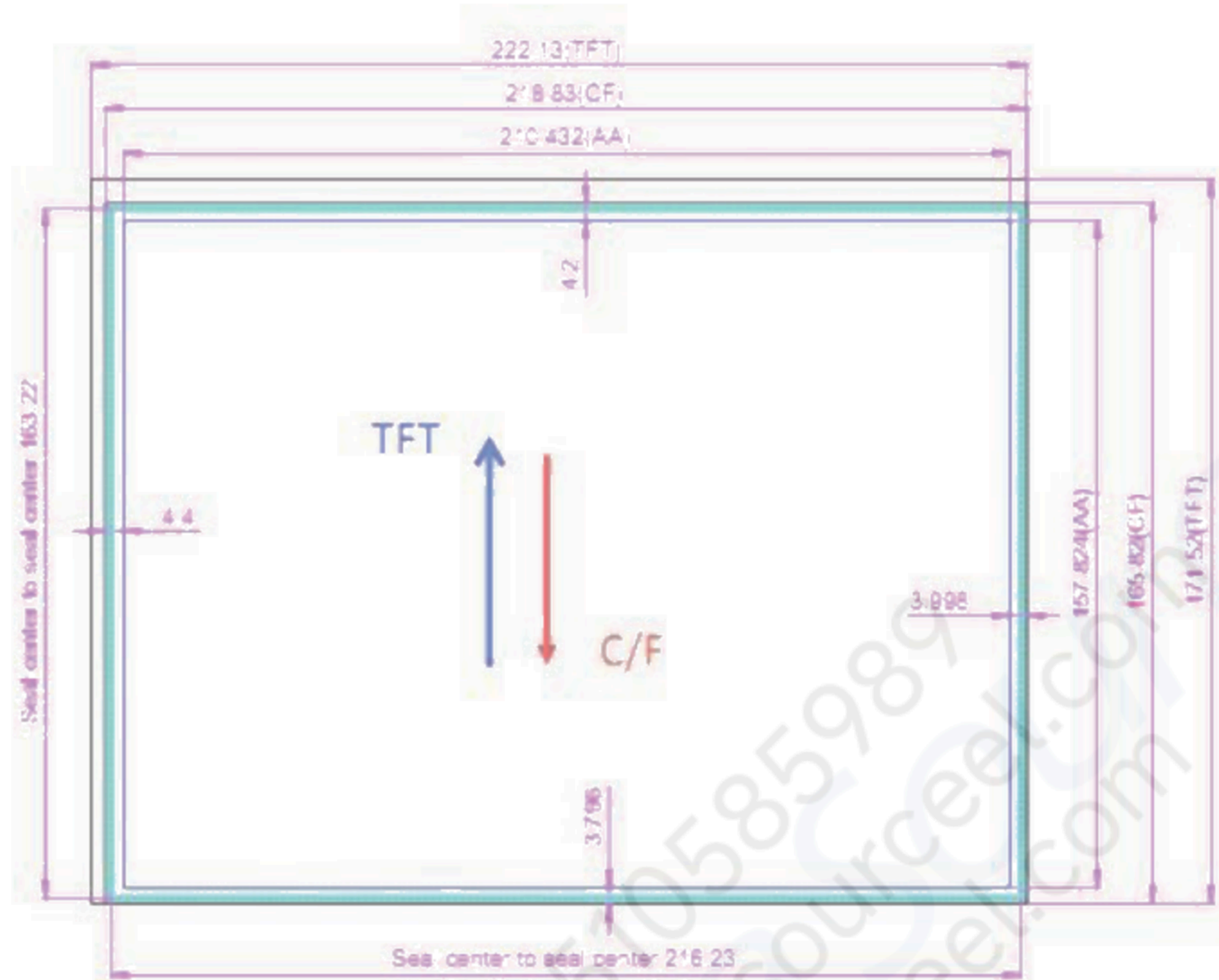
Figure 2. The TFT and CF Align Direction
