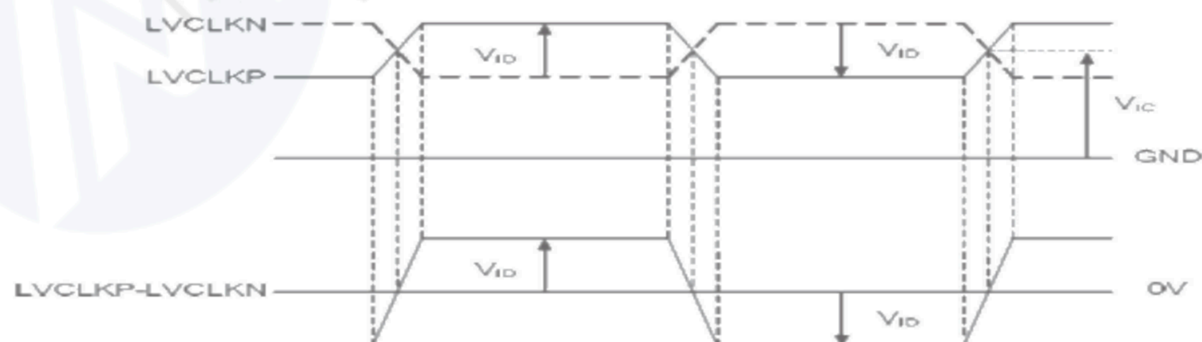
Figure 3. LVDS Signal Electrical Characteristics
