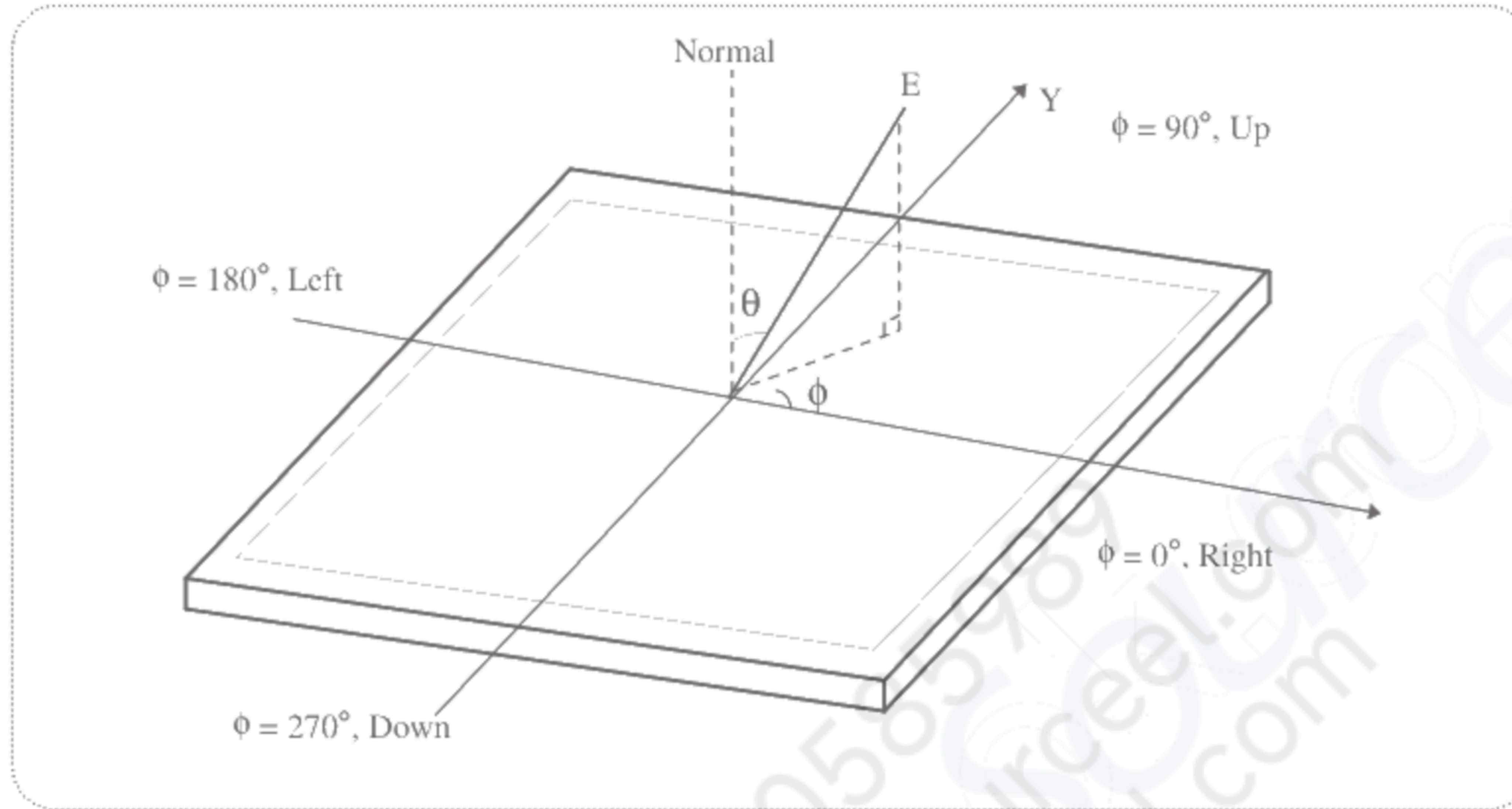
FIG.10 Viewing angle
