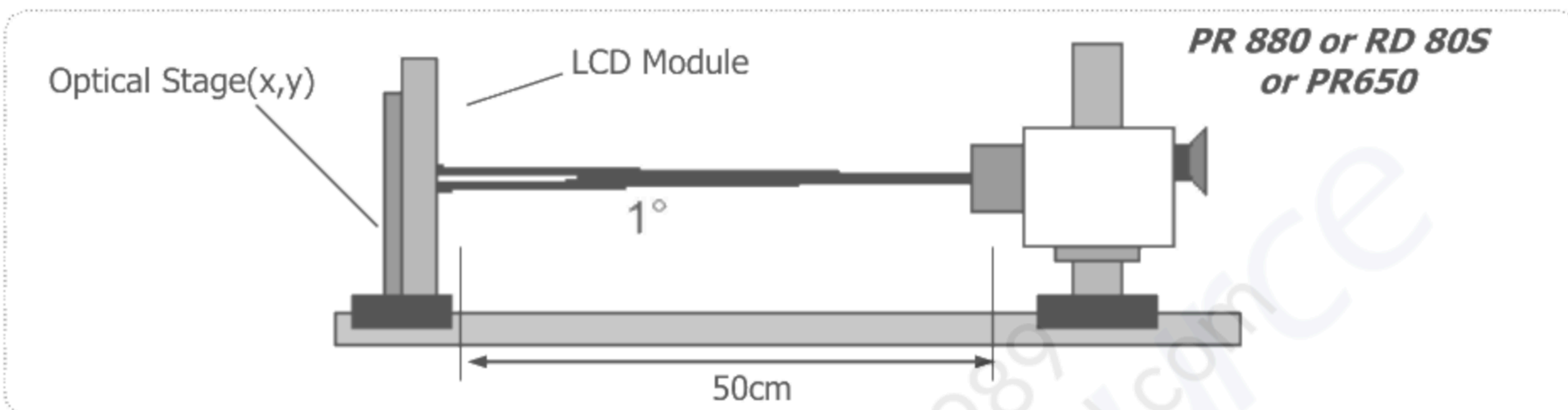
FIG.8 Optical Characteristic Measurement Equipment and Method
