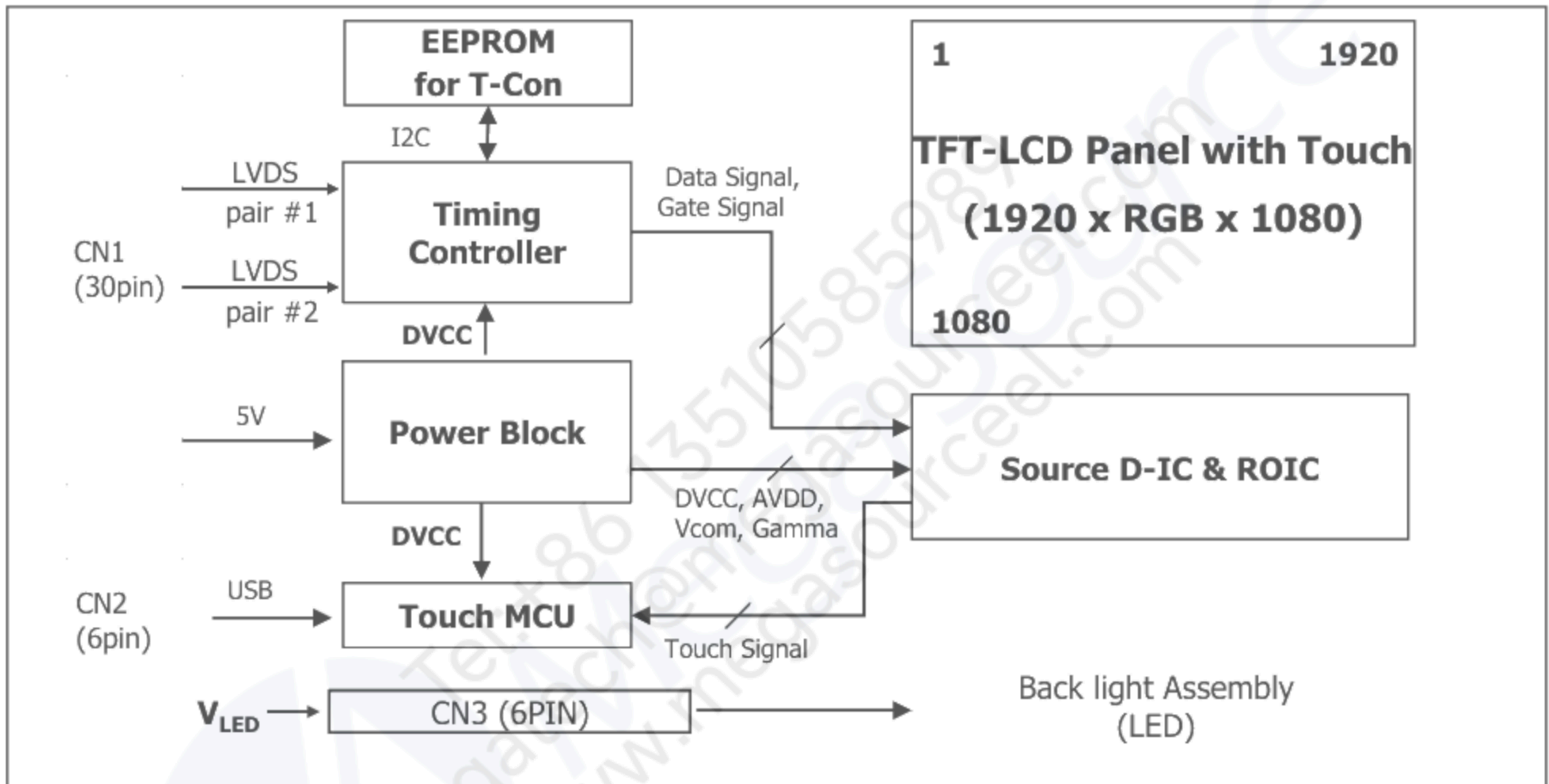
[ FIG. 1 ] Block diagram
