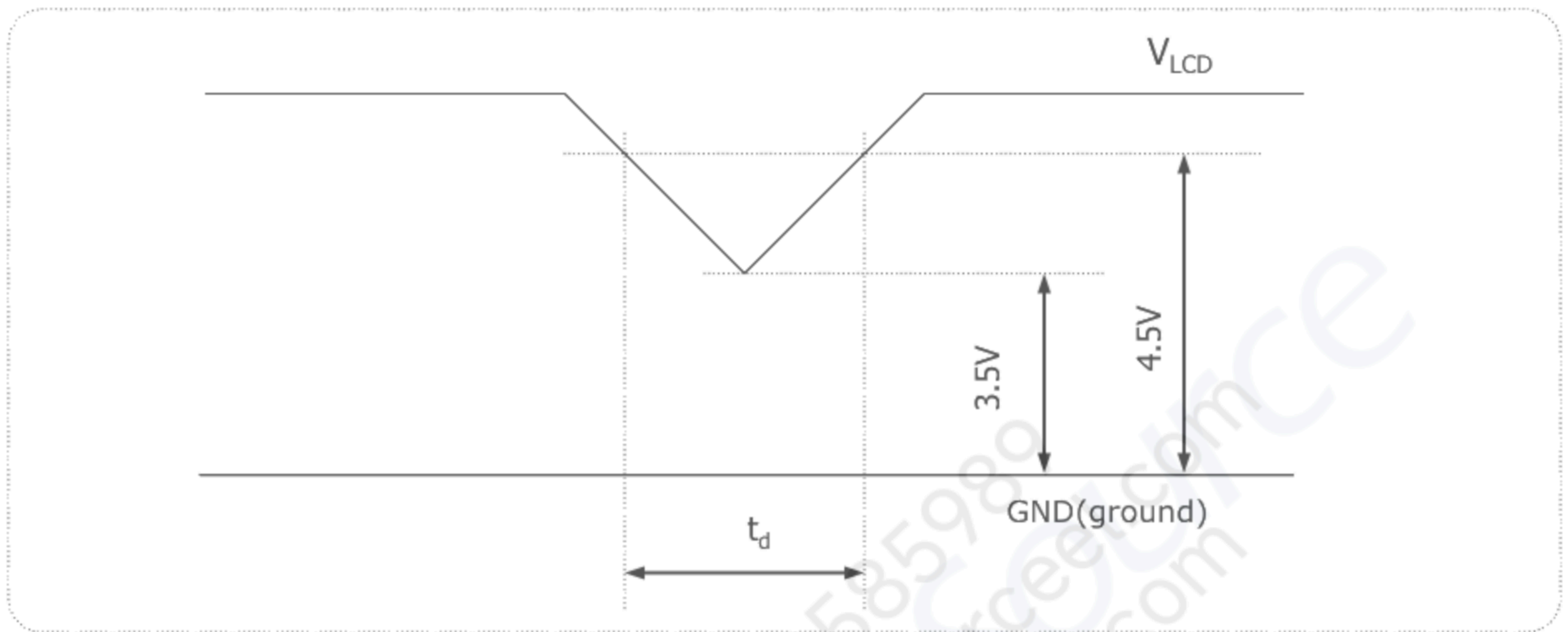
[FIG. 7] Power dip condition
