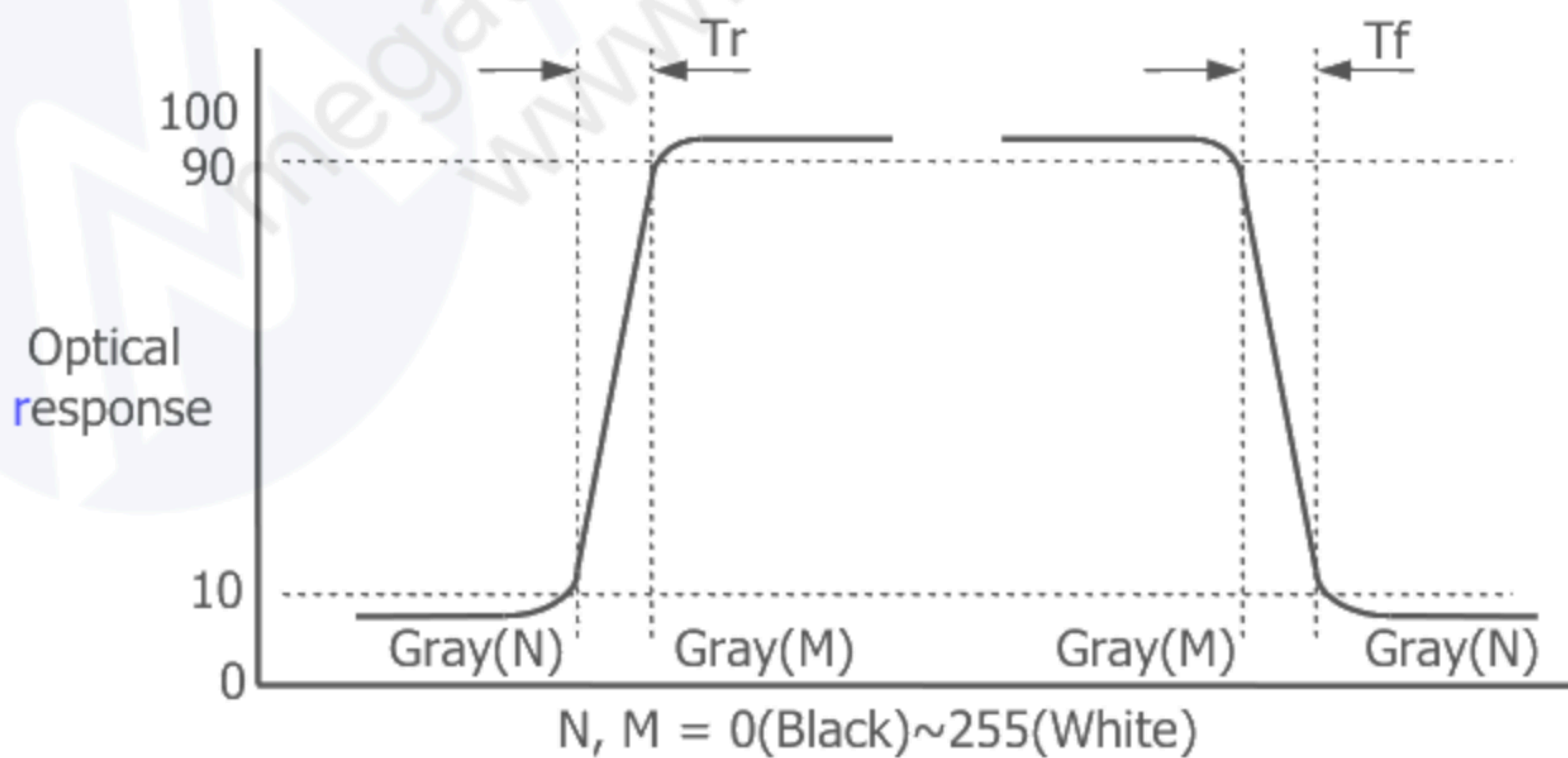
[FIG. 10] Response Time
