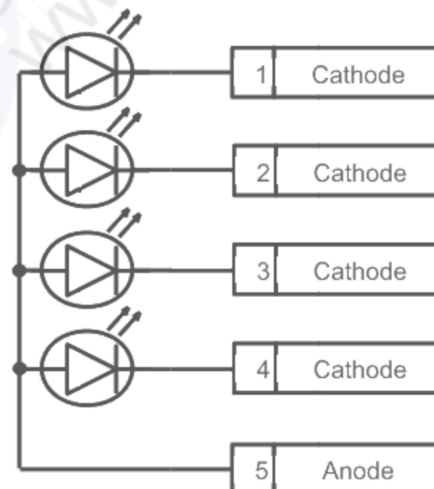
Circuit of Backlight with white LED
