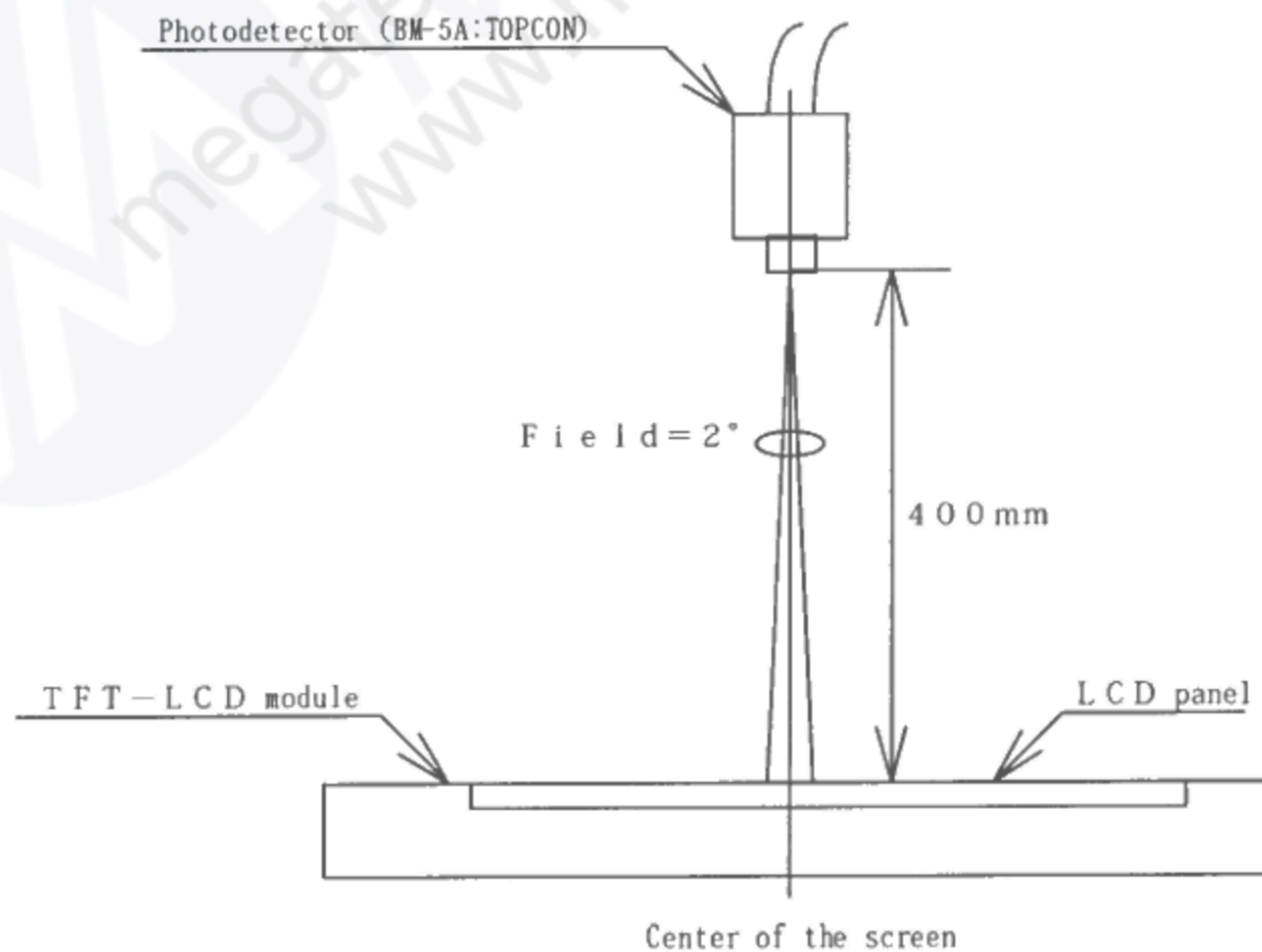
Fig.3 Optical characteristics measurement method
