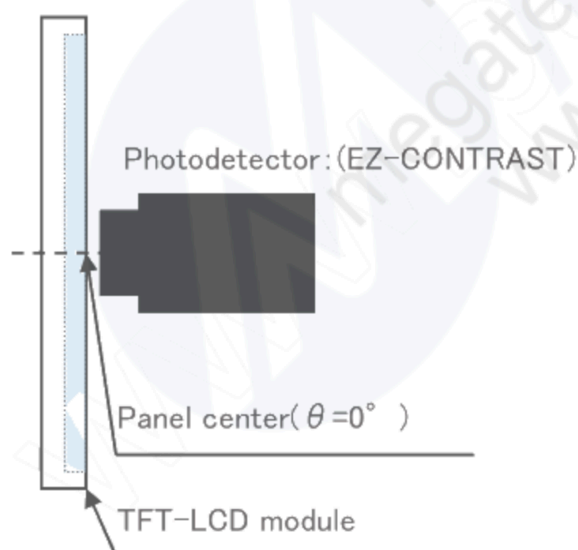
fig.2-1 Measuring method of Viewing angle range.
