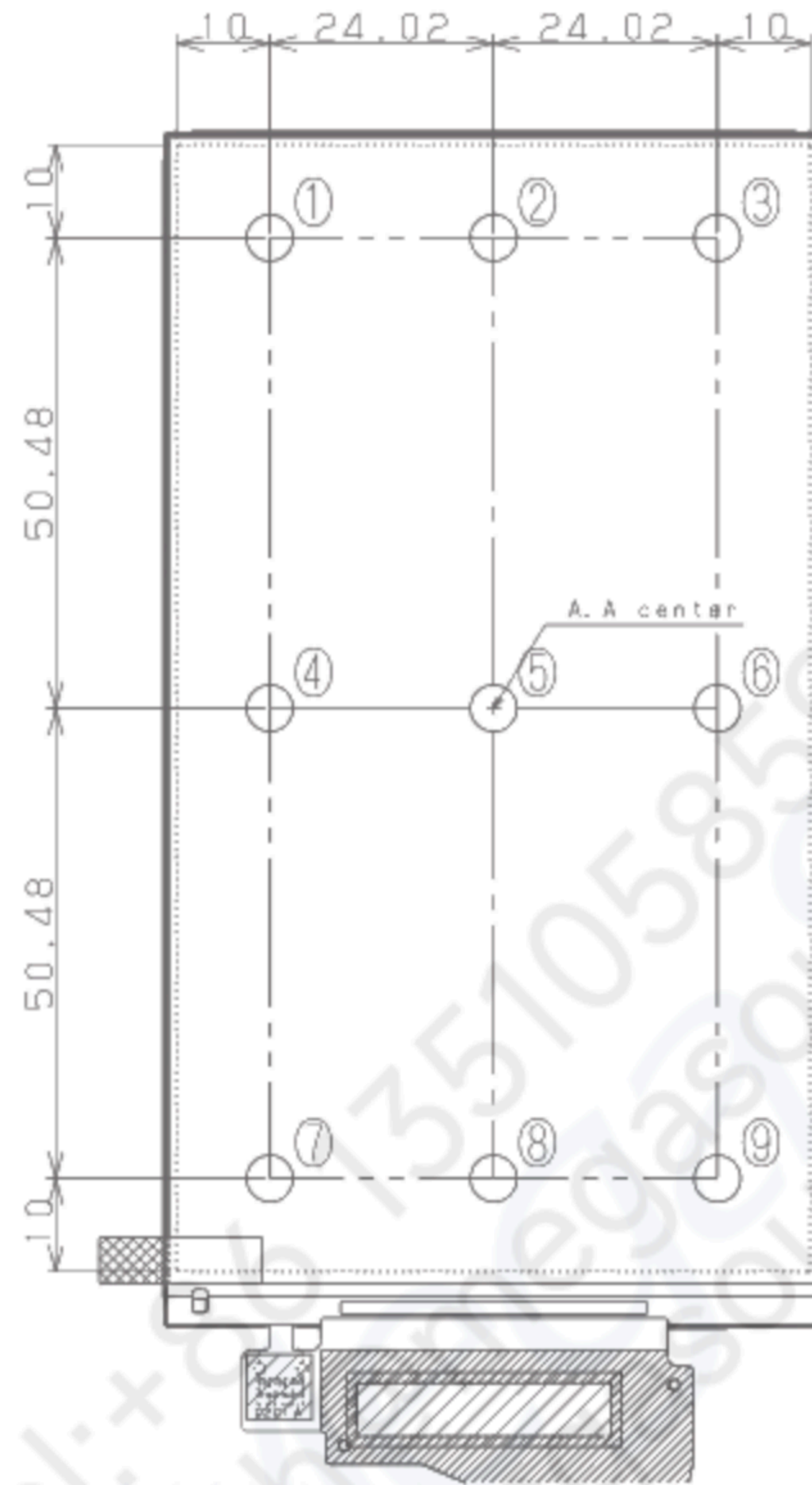
Fig. 9 Measuring Point
