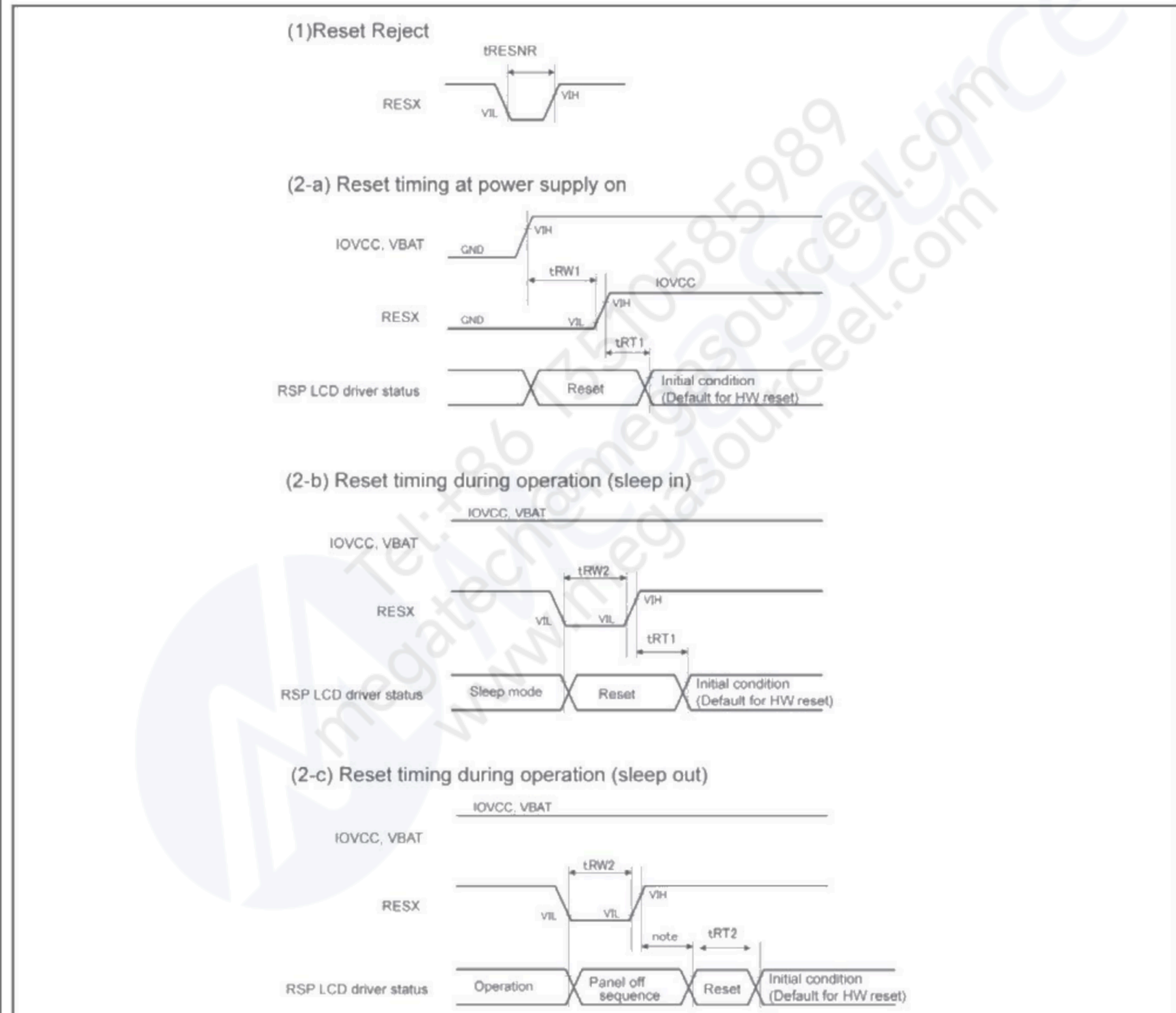
Fig .6 Reset timing characteristics
