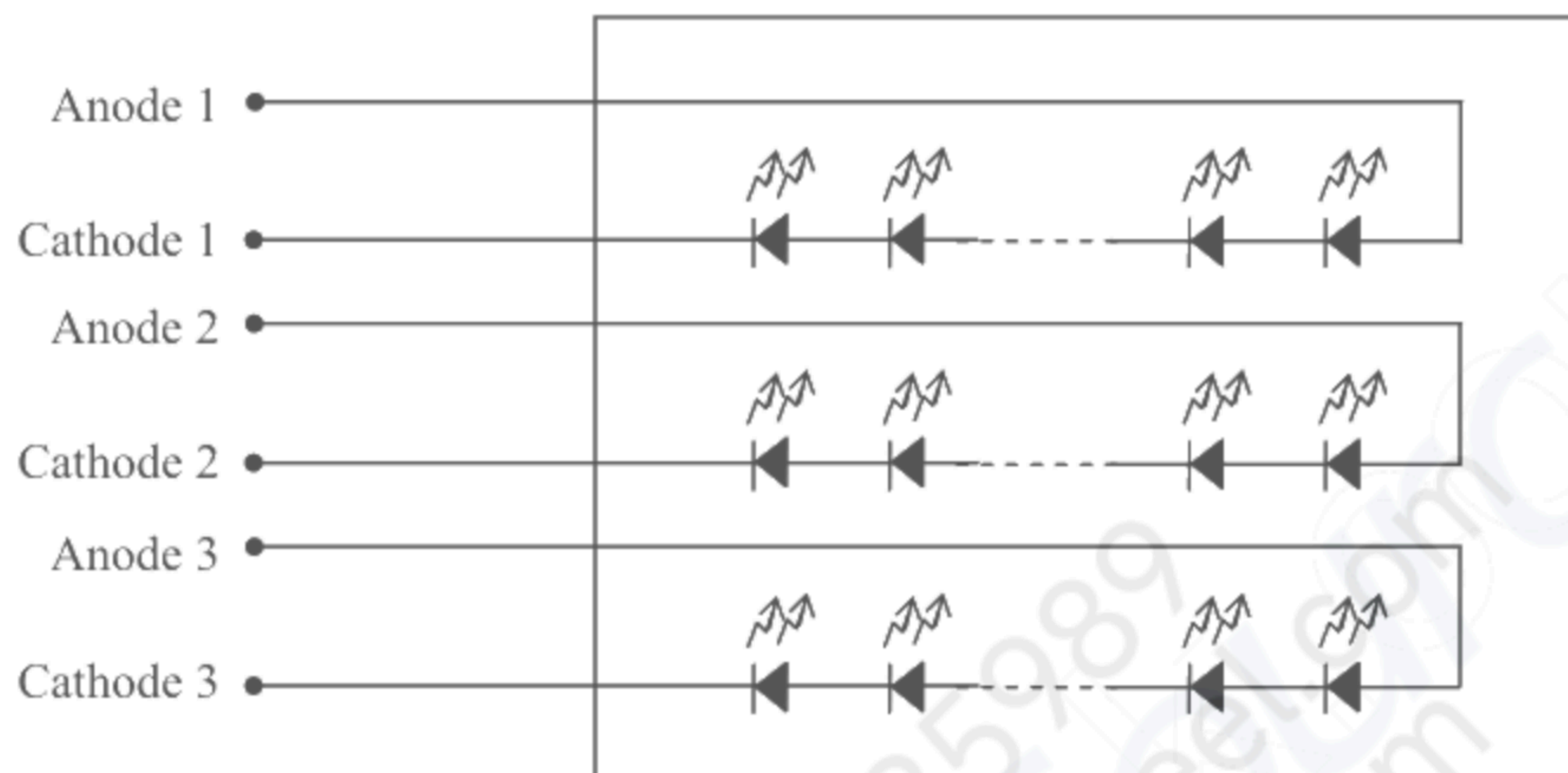
Backlight
