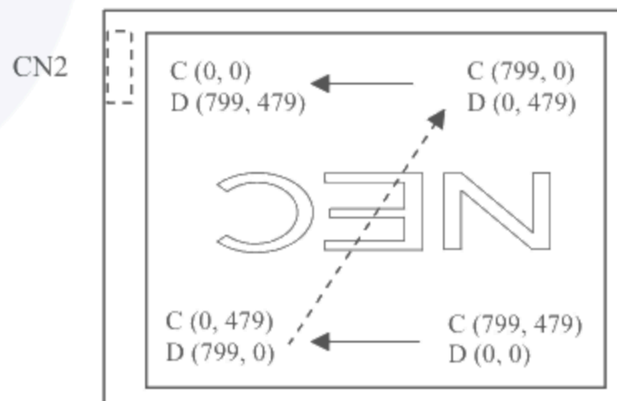
Figure2. Reverse scan (DPS: High)
