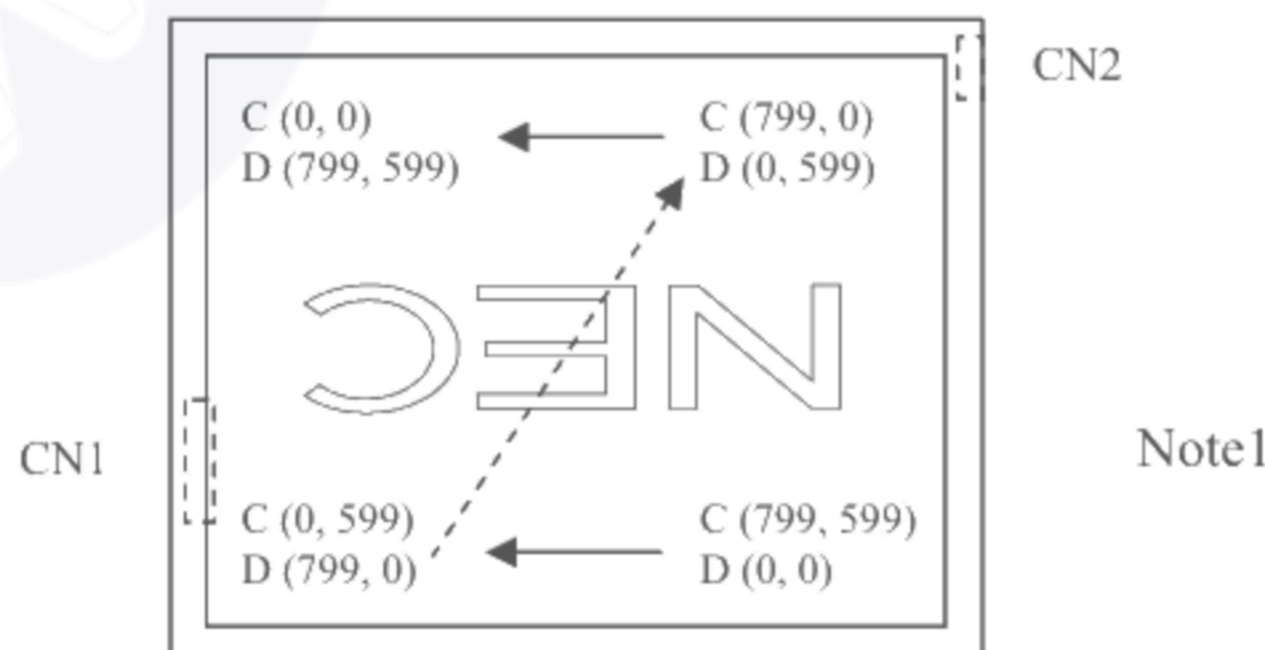
Figure2. Reverse scan (DPS: High)
