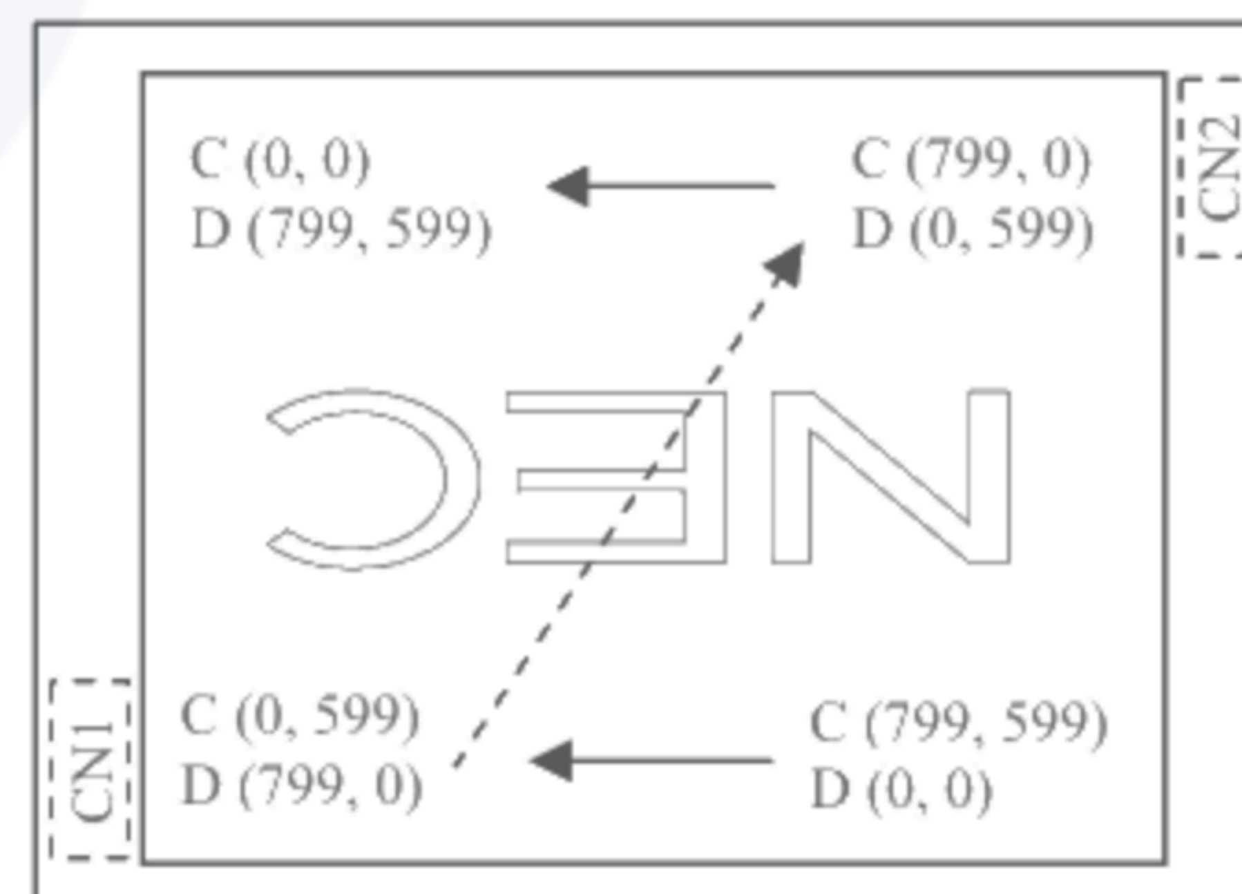
Figure2. Reverse scan (DPS: High)
