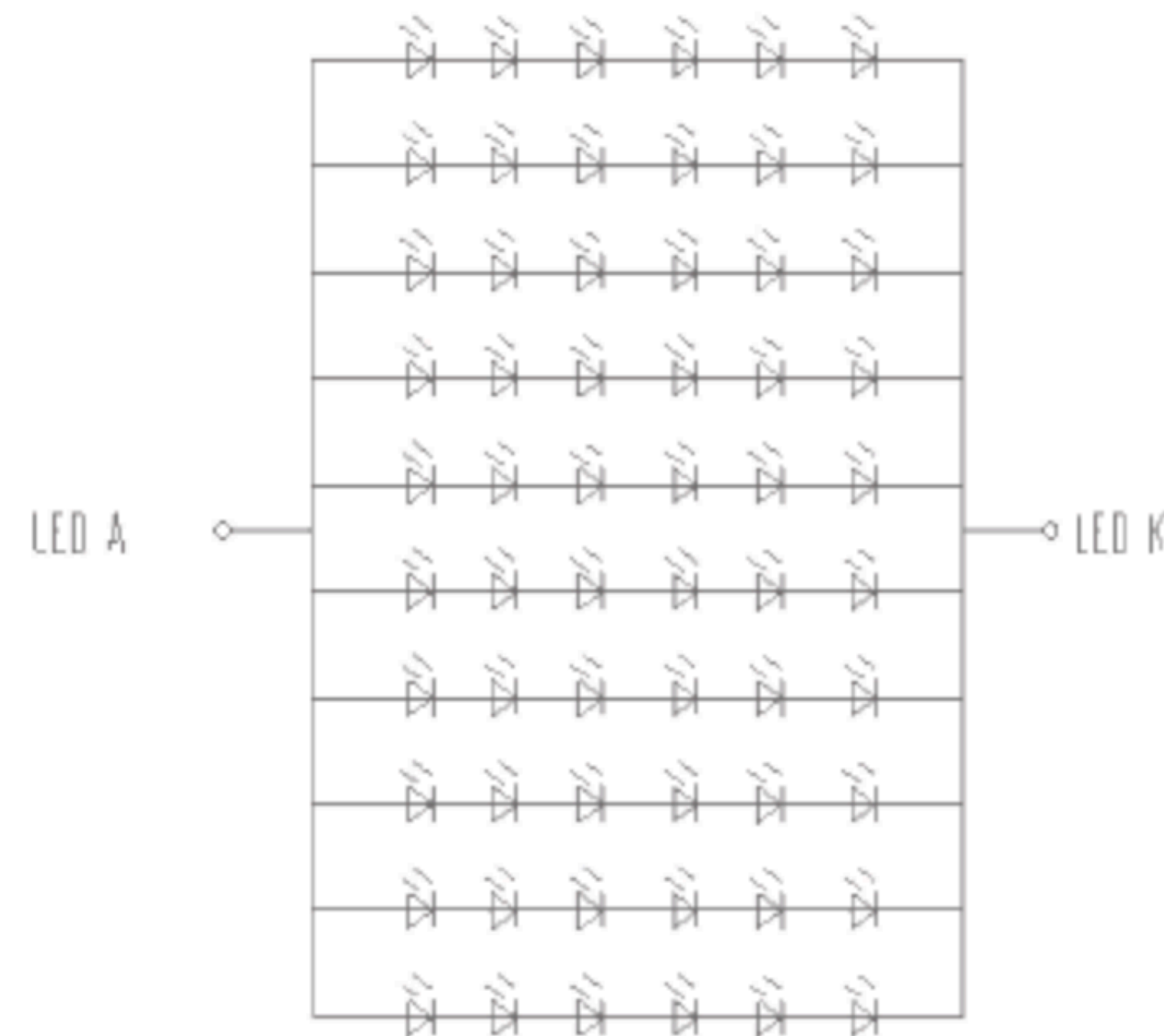
Backlight Circuit Diagram 6S-10P; If=100mA/LED
