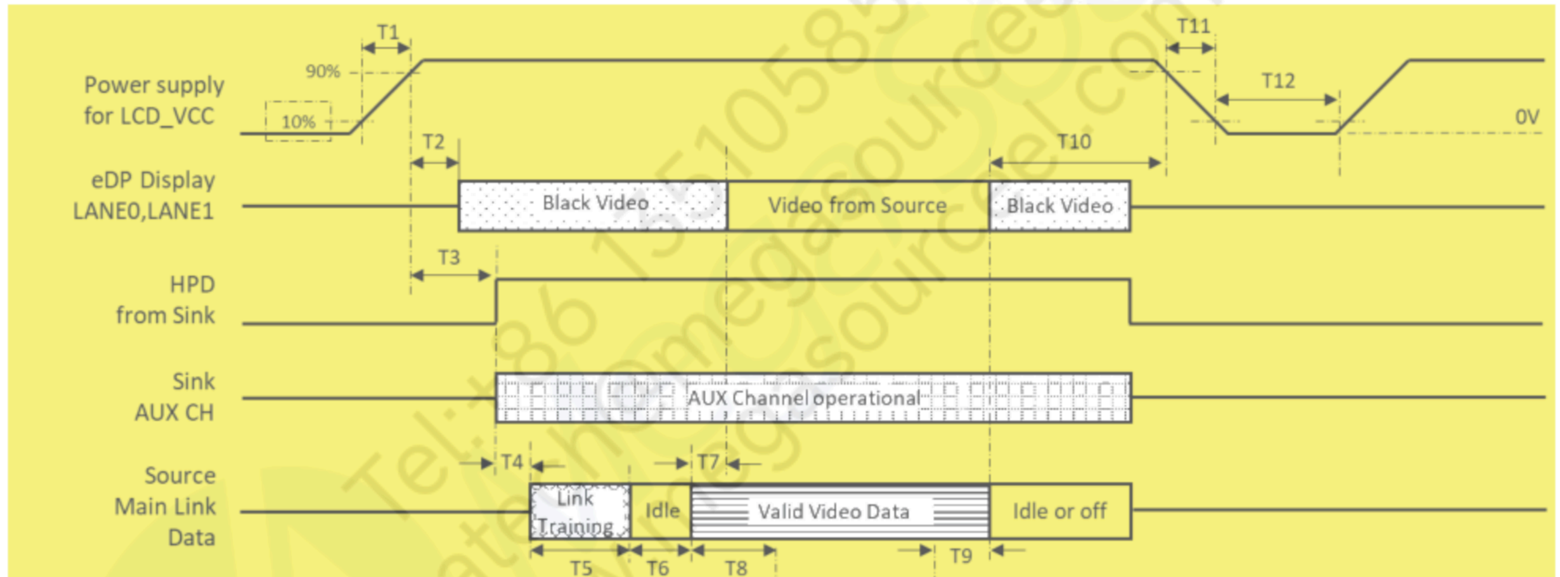
Figure 5.3.1 Power on sequence
