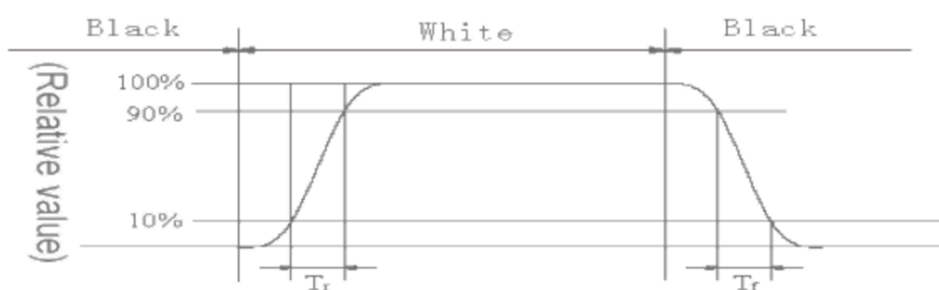
Fig3. Response Time Testing
