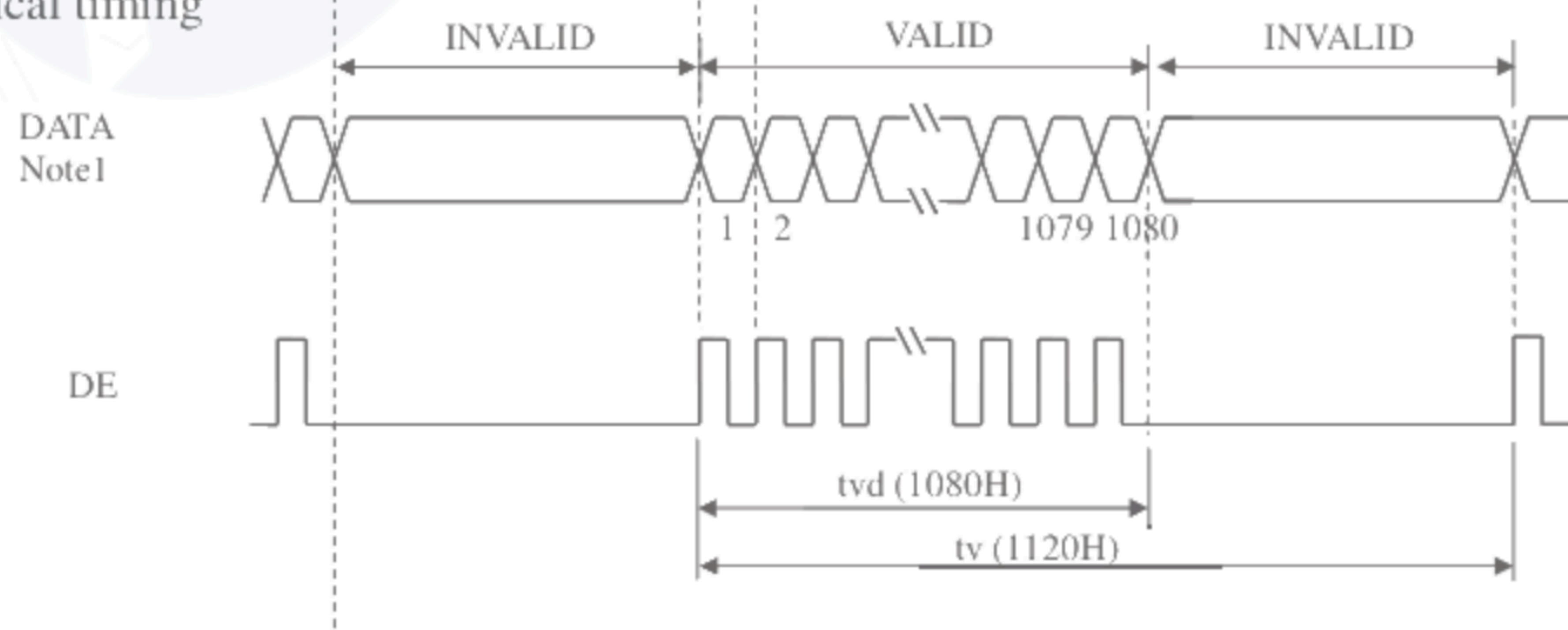
Figure 6.1.1 Input Signal Timings
