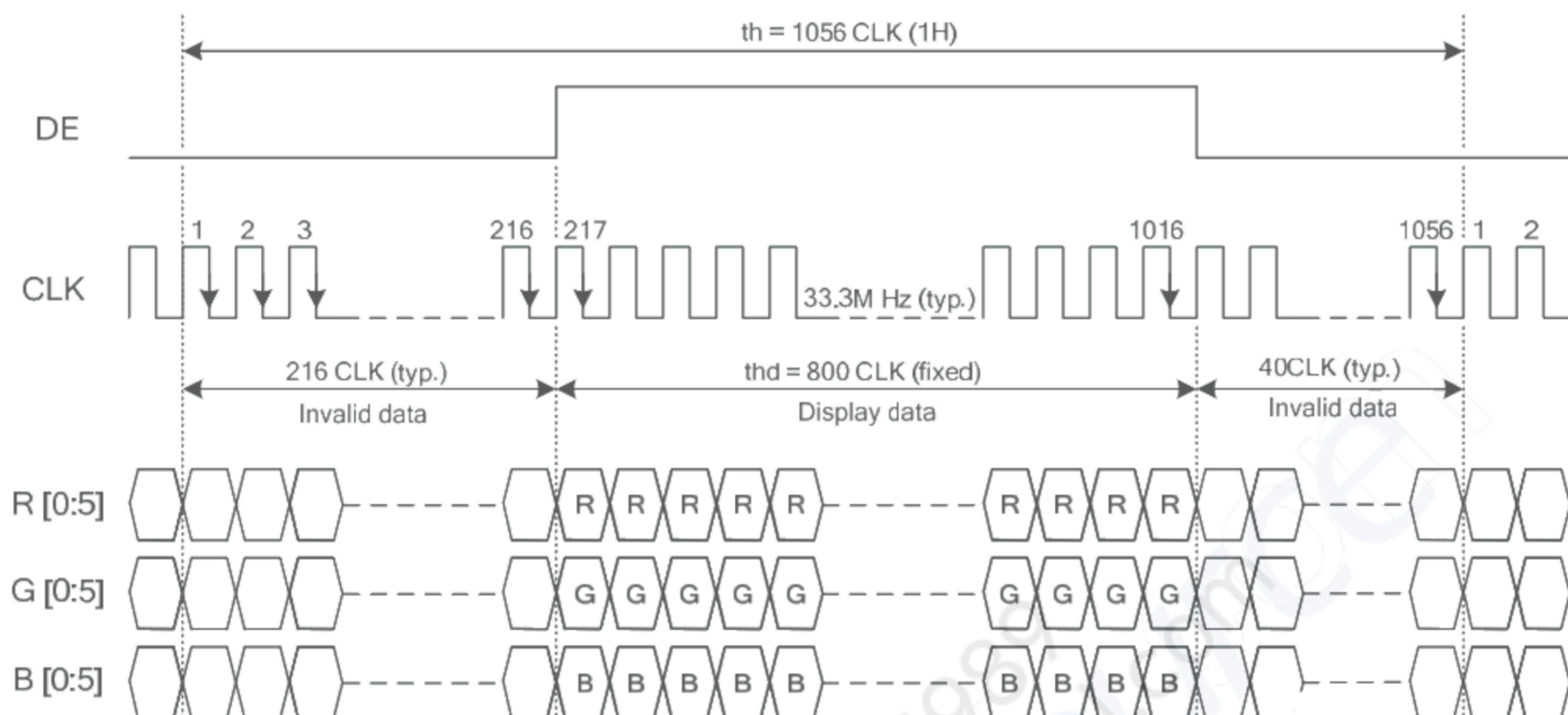
Fig. 9.1 Horizontal Timing
