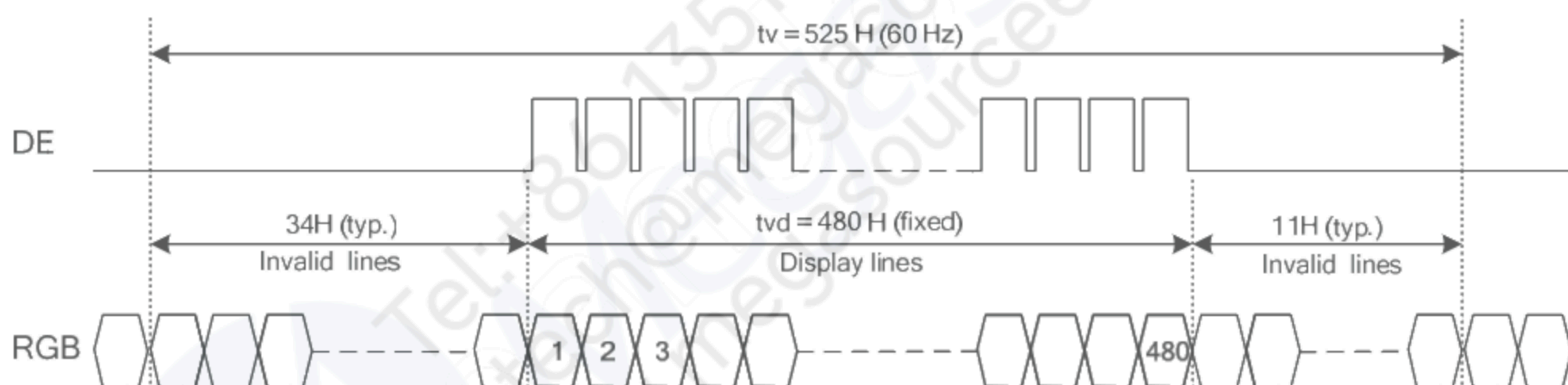
Fig. 9.2 Vertical Timing
